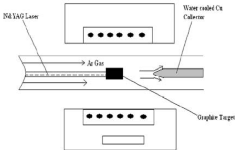
Figure 8 Laser ablation method [12]
