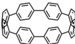
Figure 6 Cycloparaphenylene [3]
