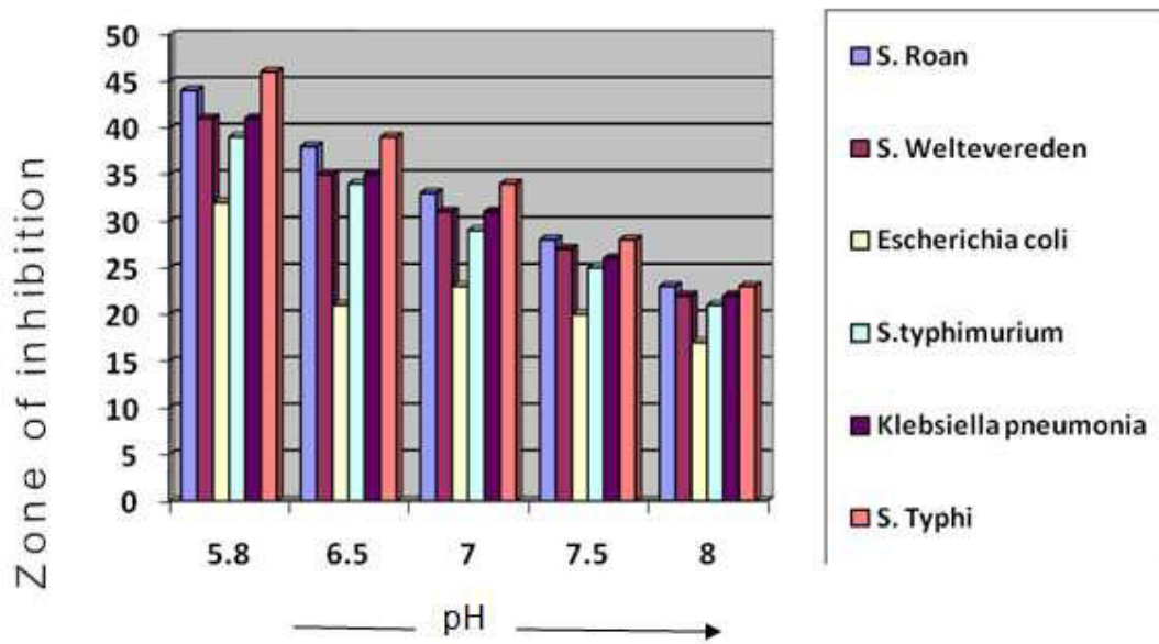
Figure3 Effect of pH on the antimicrobial activity of allicin
