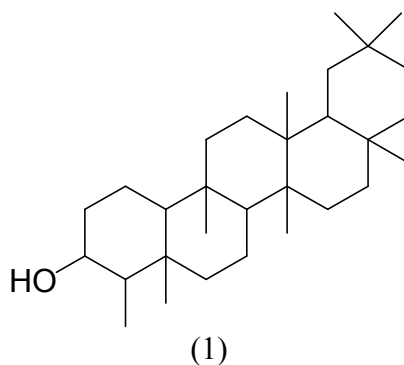
Figure 1 Friedelinol
