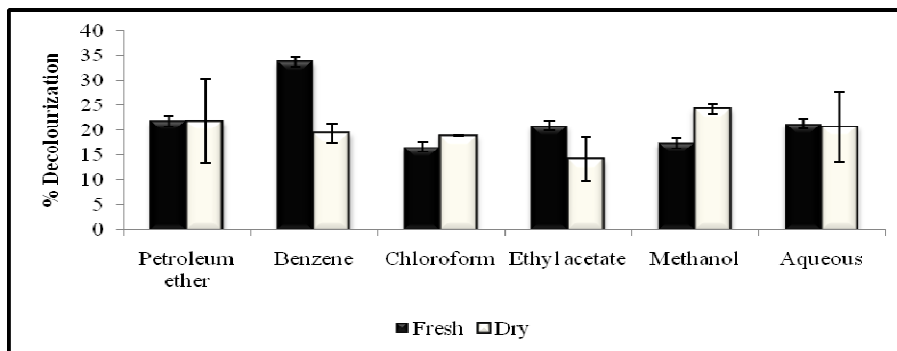
Figure 2 ABTS scavenging activity
